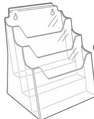
Order No. LD4101 A5 Leaflet Dispenser (4 Tier) Width 155mm Depth 34mm Height 170mm
